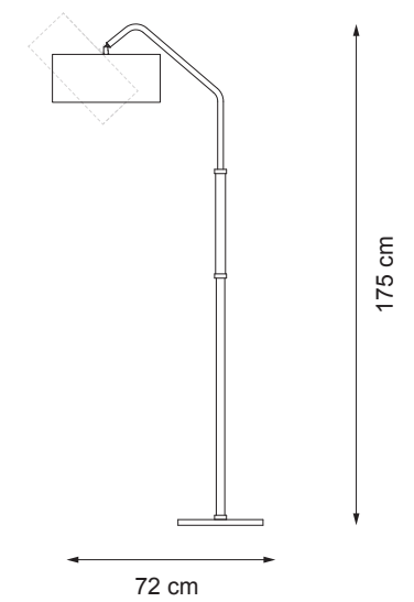
Item D08 1 light floor lamp (E27)
