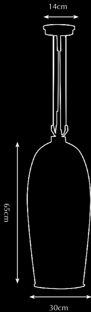
Itemnr: PA 825 Model: Rosedale hanging lamp long Material: Casted brass/Blown glass Socket: E27 max. 60Watt Finishes: -Dutch Silver -Canadian Gold -Rose Gold
