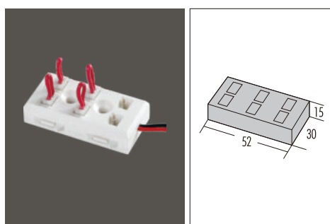
Connector
