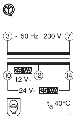
TS25/12-24 C
