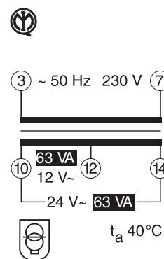
TS63/12-24 C
