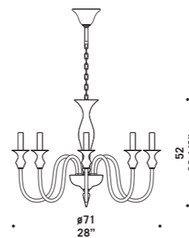
2599 K8 8 x max 46W E14 HSGSB/C/UB alogeno chiara clear halogen 8 x E14 LED LED light bulb
