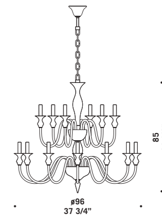
2599 K12+6 18 x max 46W E14 HSGSB/C/UB alogeno chiara clear halogen 18 x E14 LED LED light bulb
