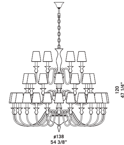
2599 K24+12+6 SHADE 42 x max 46W E14 HSGSB/C/UB alogena chiara clear halogen 42 x E14 LED LED light bulb
