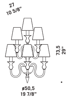
2599 A6 SHADE 6 x max 46W E14 HSGSB/C/UB alogena chiara clear halogen 6 x E14 LED LED light bulb
