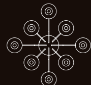
Art. 1710/CH8/KR/RS/V2 ø 86 cm H 80 cm Pø 14 cm 8 x E14 x 25W
