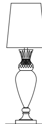
Art. 1953/P Pø 26 cm H 82 cm 1 x E27 x 40W
