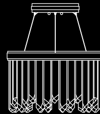
888140-x (LED QTY 12) H. 13.5" (34 cm) W. 21" (53 cm) UP: Min Ht. X" (X cm) Max Ht. 98" (249 cm) DOWN: Min Ht. 22" (56 cm) Max Ht. 110" (279 cm)
