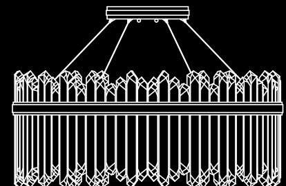
882840-x H. 18.5" (47 cm) W. 41" (104 cm) Min Ht. 38" (97 cm) Max Ht. 110" (279 cm) (LED QTY 48)
