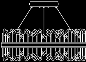
882040-x H. 12" (30 cm) W. 21" (53 cm) Min Ht. 16" (41 cm) Max Ht. 104" (264 cm) (LED QTY 24)
