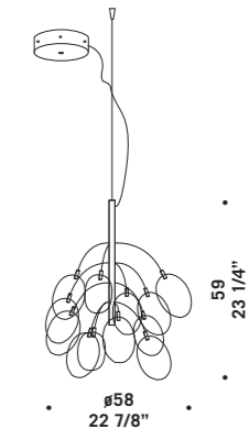
PRO•SECCO S13D 13x20W-12V G4 HSGST/UB alogeno bispina halogen bi-pin cavo elettrico 150 cm trasform. elettr. dimmerabile cables lenght 150 cm electronic transf. dimmable
