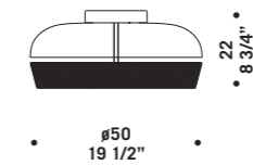
DOME P50 27W 2520lm LED 2700K CRI90
