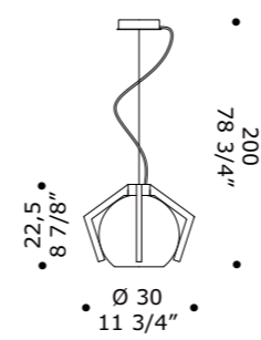
<TAG> S/S1D 1 x 15W E27 LED LED light bulb CE IP 20
