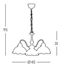
731.83.116 Luster/chandelier ☑ 3 lp., E27, 75 W
