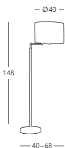
1264.41.6 Bodenleuchte / floor lamp 1 Ip., E27, 60 W vernickelt / nickel plated
