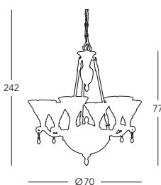
206.86+2 Luster/chandelier ☑ 8 lp., E27, 60 W
