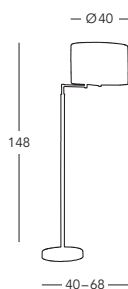
1264.41.7 Bodenleuchte / floor lamp 1 Ip., E27, 60 W messing / brass
