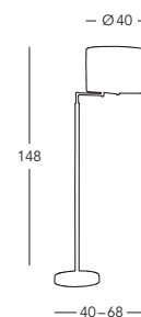
1264.41.4 Bodenleuchte / floor lamp 1 Ip., E27, 60 W altmessing / antique brass
