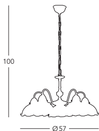
731.85.110 Luster/chandelier 5 lp., E27, 75 W
