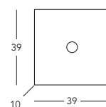
0342.14.3 Deckenleuchte/ ceiling lamp ☑ 4 lp., E27, 60 W
