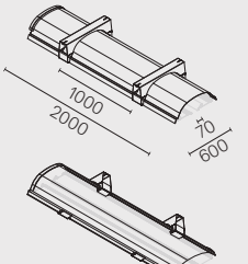
Bóveda de Composite Composite Housing
